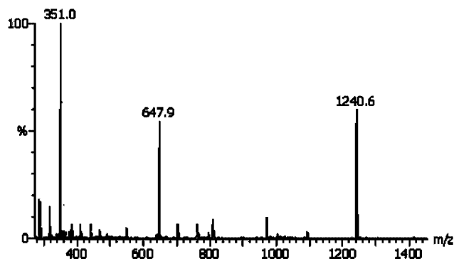
Figure 1. ESI mass spectrum (negative ions) of (PNP)_4[Co_4(1)_4] ( 7 ).
